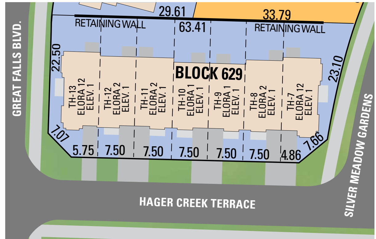
BLOCK 629 SITE PLAN
